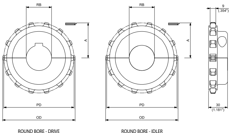
ROUND BORE - DRIVE
