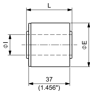
STANDARD ROLLER
