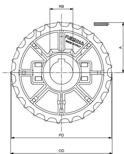
ROUND BORE - DRIVE
