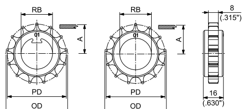
ROUND BORE - DRIVE
