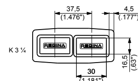
RUBBER PAD POSITION
