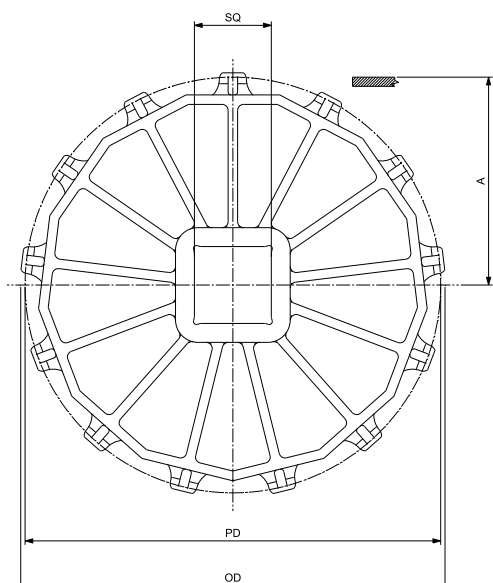
SQUARE BORE - DRIVE/IDLER
