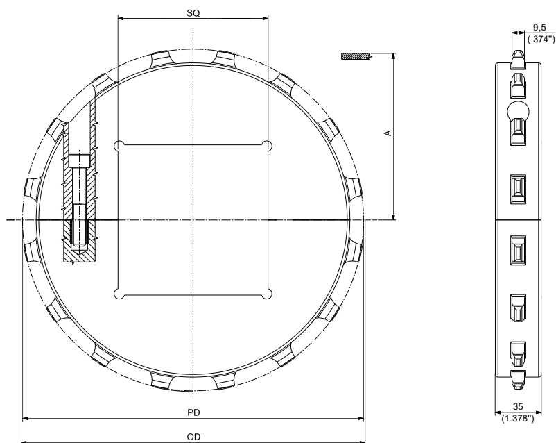
SQUARE BORE - DRIVE/IDLER
