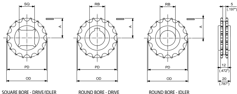
SQUARE BORE - DRIVE/IDLER
