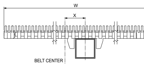
TRACKING GUIDE LOCATION
