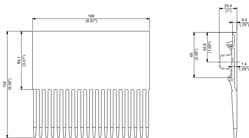
PART NUMBER TC1500-01
