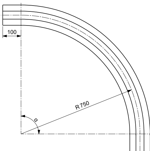
Radius
